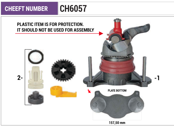
Caliper Mechanism Set (MB Trailer Axle) OEM NUMBER
