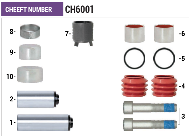
Caliper Guides & Seals Repair Kit OEM NUMBER SF MODUL T SF 3 434 3861 00 - KRONE 550017811 HALDEX 95397 - HALDEX 95054 - JOST Axle JAE0250410063 - GIGANT 716080004 - 703011013 - 16030004 - SCANIA 2305913 - 2092720
