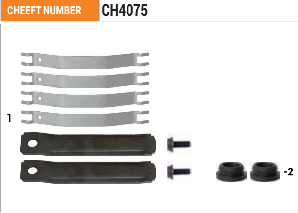
Caliper Pad Retainer Repair Kit OEM NUMBER -SAF 3 434 3851 01 -RENAULT 5021 174 162 - 5021 174 180 -HALDEX 94659 - HENDRICKSON S-30560-03
